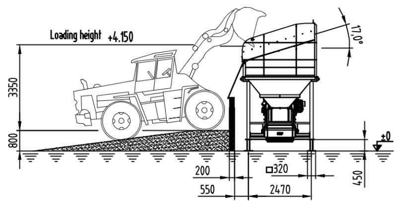
Section Y-Y - Rap Feed
