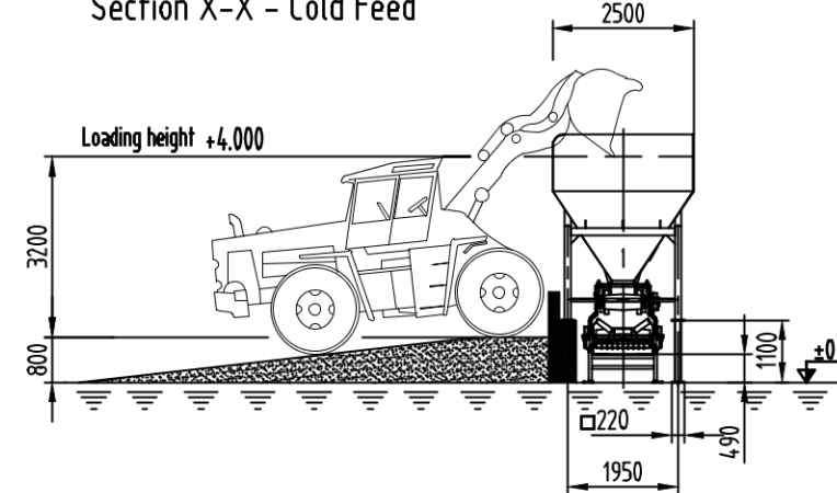
Section X-X - Cold Feed
