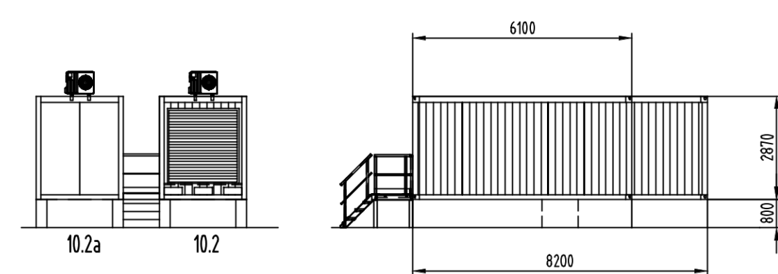
View on C
